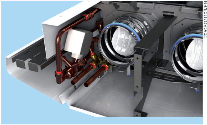
Water valves and adjustment damper
